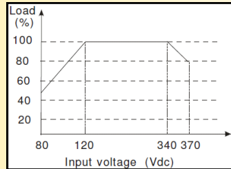
Output power characteristics as a function of the input voltage standard AL140L version
